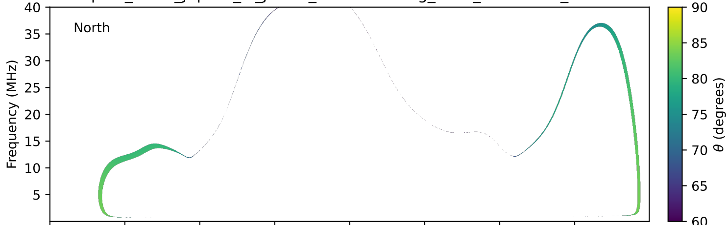
expres_earth_jupiter_io_jrm33_lossc-wid1deg_3kev_20240327_v11.cdf
