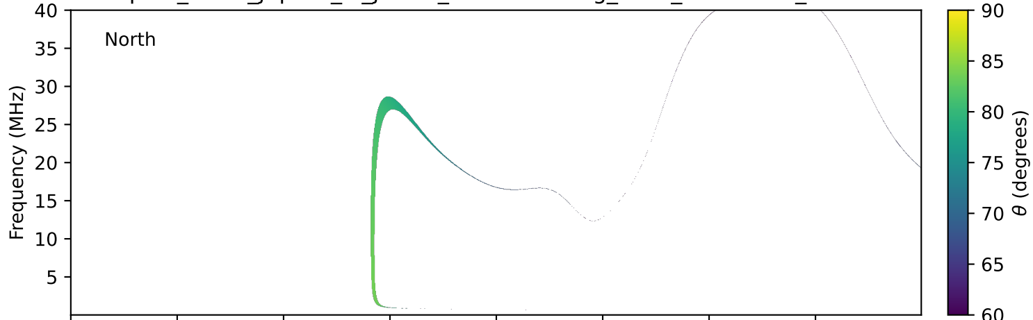
expres_earth_jupiter_io_jrm33_lossc-wid1deg_3kev_20240325_v11.cdf
