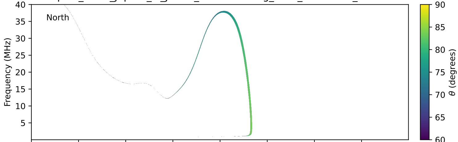
expres_earth_jupiter_io_jrm33_lossc-wid1deg_3kev_20240315_v11.cdf
