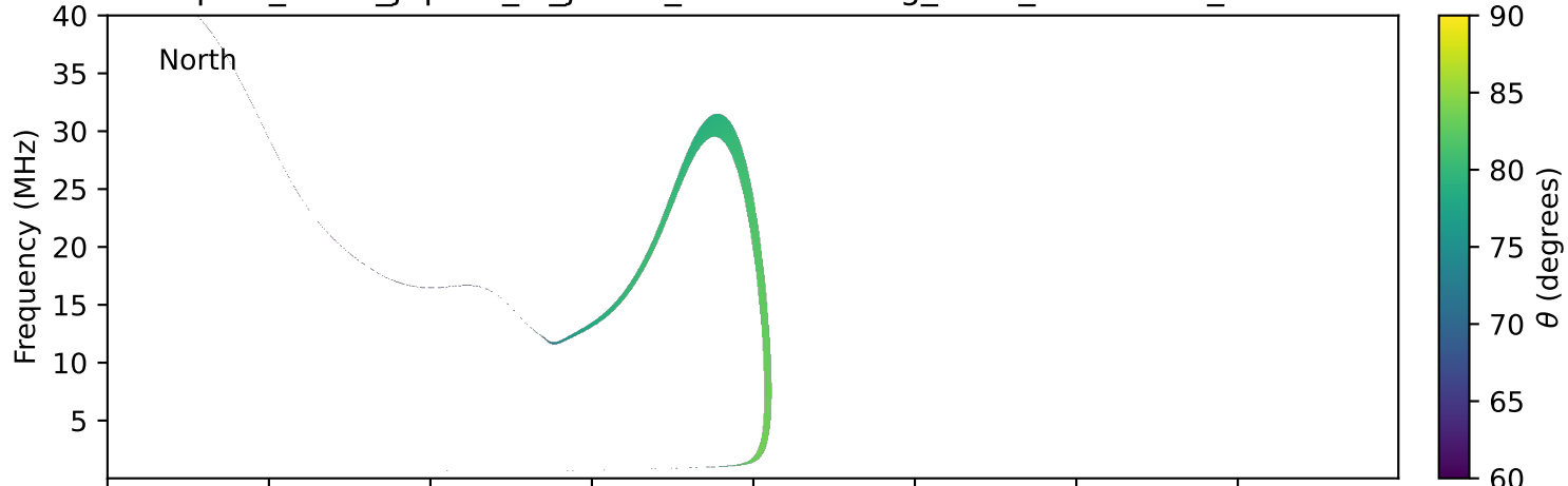
expres_earth_jupiter_io_jrm33_lossc-wid1deg_3kev_20240308_v11.cdf
