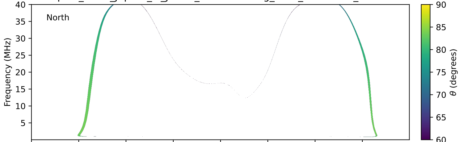
expres_earth_jupiter_io_jrm33_lossc-wid1deg_3kev_20240304_v11.cdf
