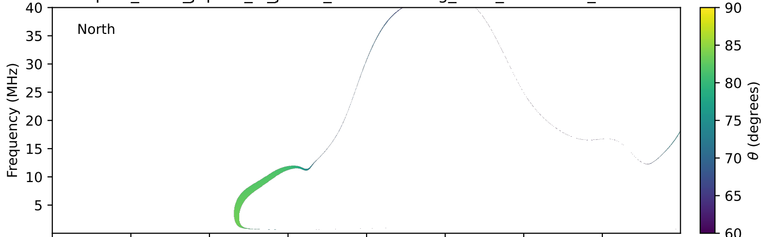
expres_earth_jupiter_io_jrm33_lossc-wid1deg_3kev_20240302_v11.cdf
