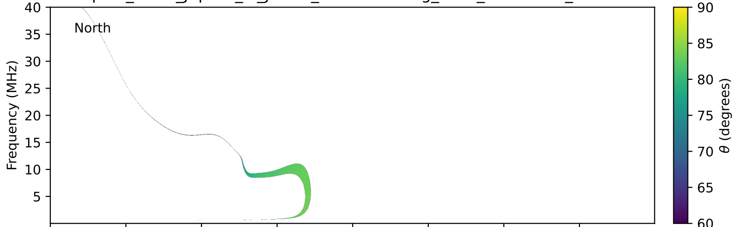
expres_earth_jupiter_io_jrm33_lossc-wid1deg_3kev_20240301_v11.cdf
