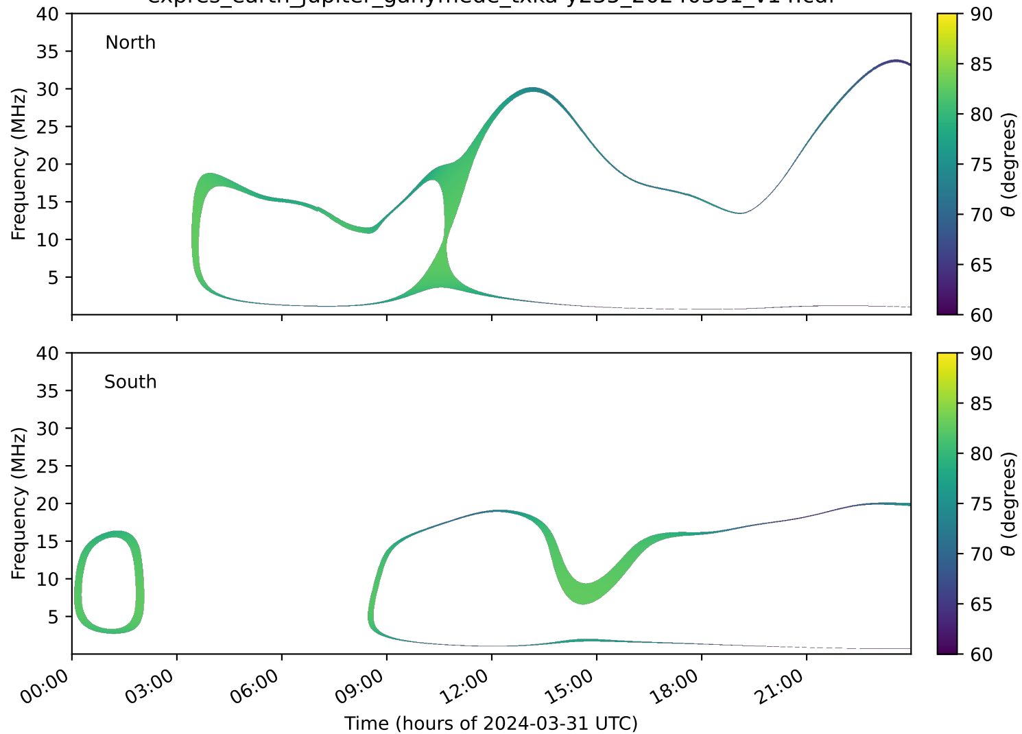
expres_earth_jupiter_ganymede_txka-y235_20240331_v14.cdf
