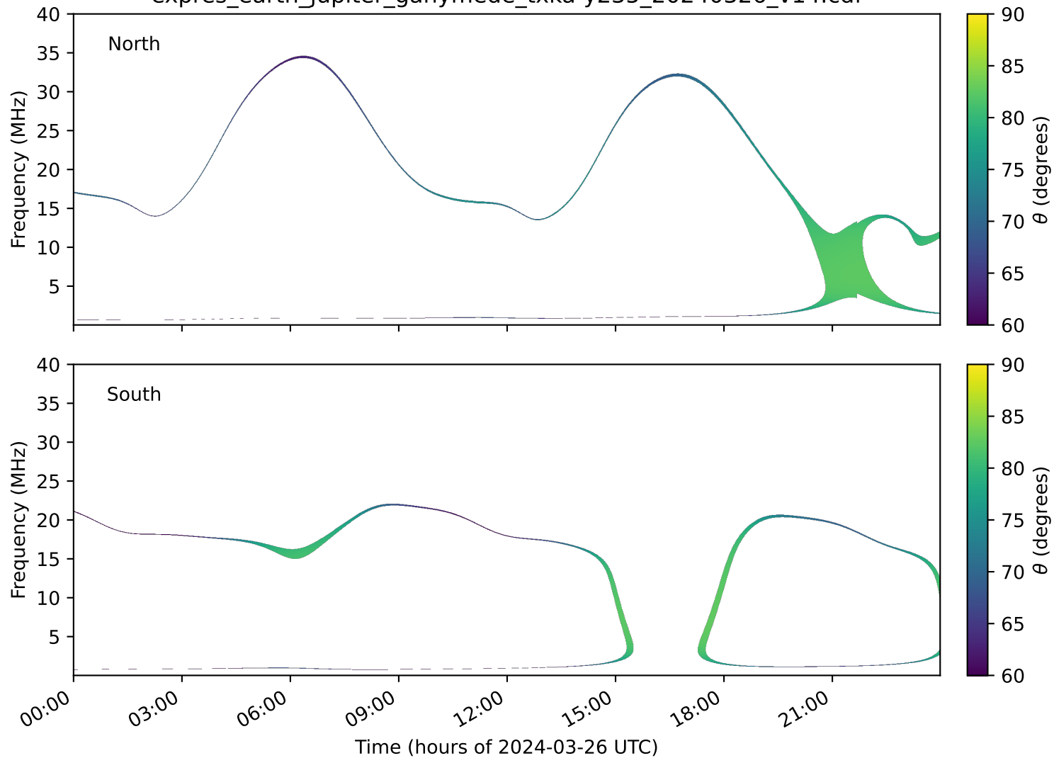
expres_earth_jupiter_ganymede_txka-y235_20240326_v14.cdf
