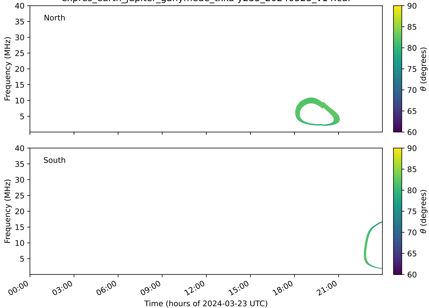
expres_earth_jupiter_ganymede_txka-y235_20240323_v14.cdf
