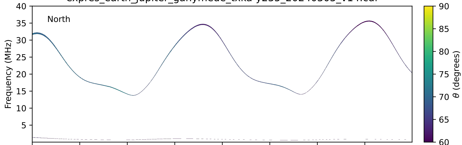
expres_earth_jupiter_ganymede_txka-y235_20240303_v14.cdf
