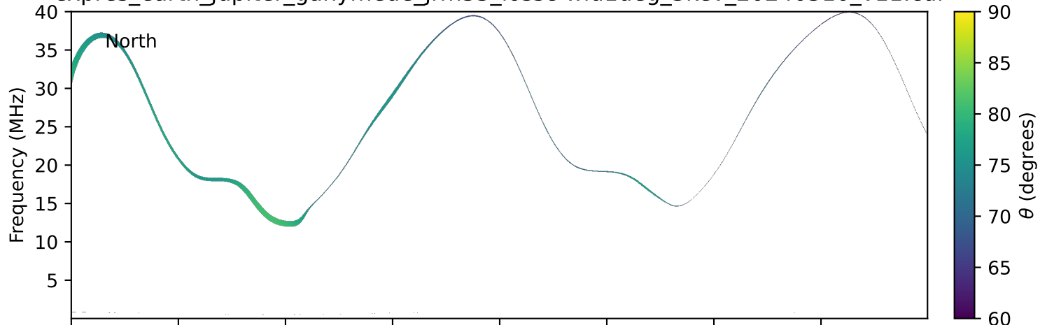
expres_earth_jupiter_ganymede_jrm33_lossc-wid1deg_3kev_20240310_v11.cdf
