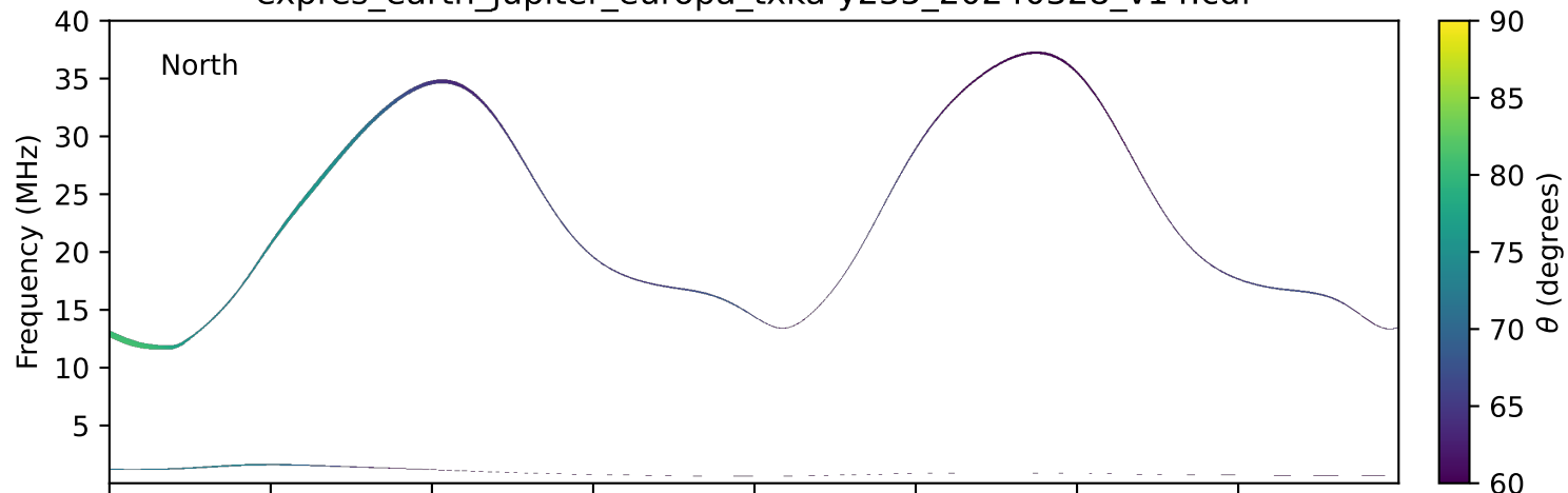
expres_earth_jupiter_europa_txka-y235_20240328_v14.cdf
