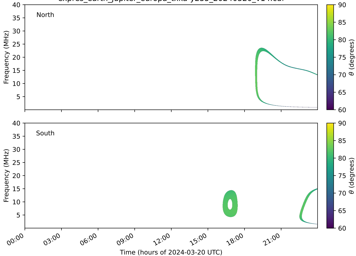
expres_earth_jupiter_europa_txka-y235_20240320_v14.cdf
