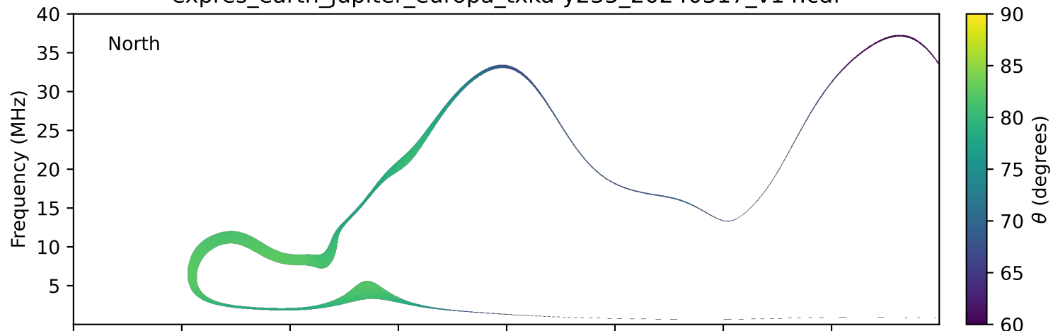
expres_earth_jupiter_europa_txka-y235_20240317_v14.cdf
