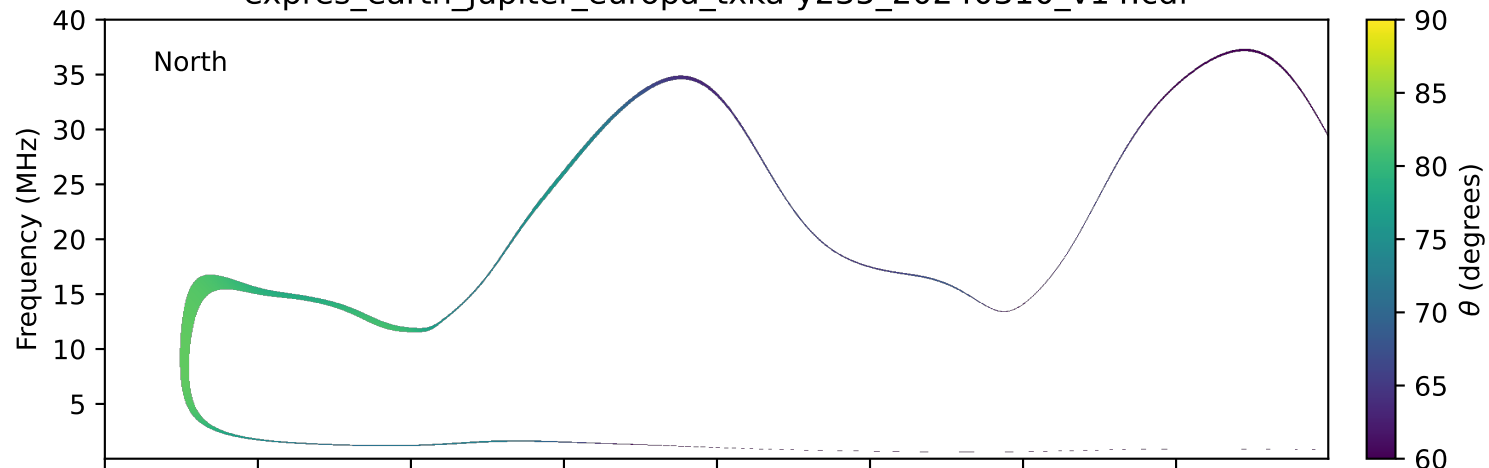
expres_earth_jupiter_europa_txka-y235_20240310_v14.cdf
