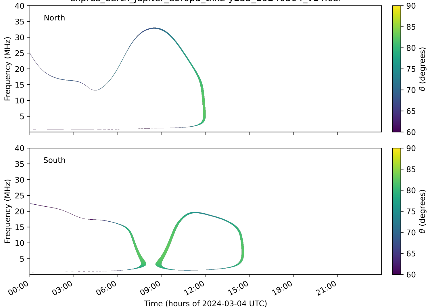
expres_earth_jupiter_europa_txka-y235_20240304_v14.cdf
