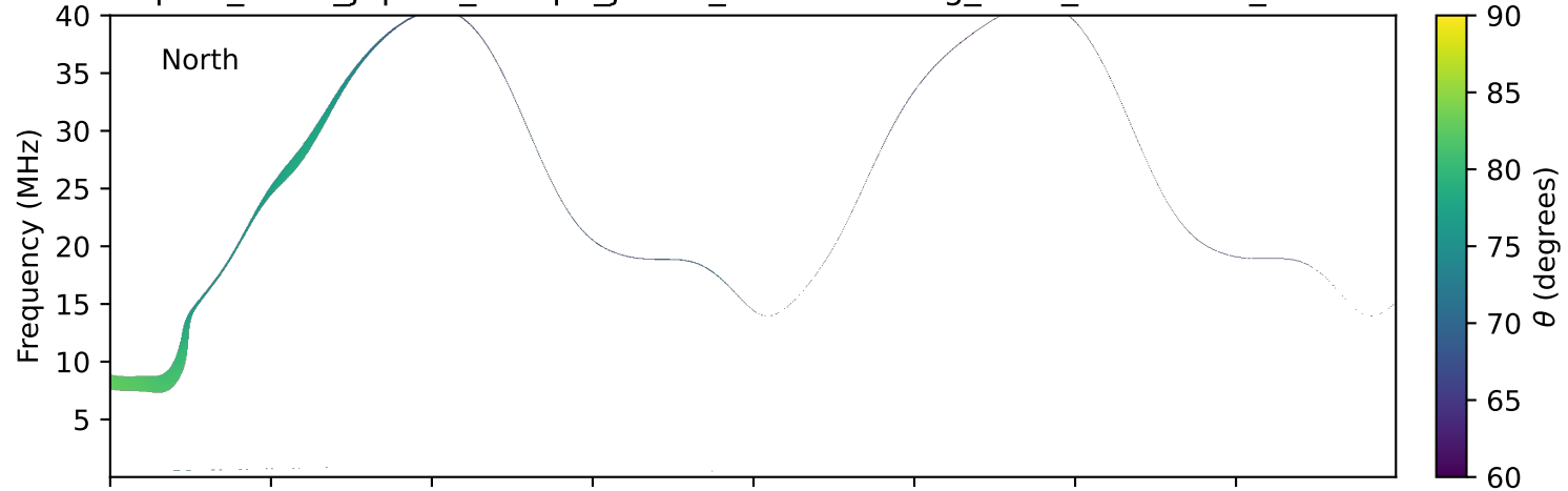
expres_earth_jupiter_europa_jrm33_lossc-wid1deg_3kev_20240328_v11.cdf
