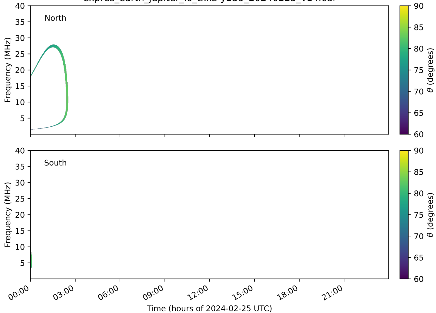
expres_earth_jupiter_io_txka-y235_20240225_v14.cdf
