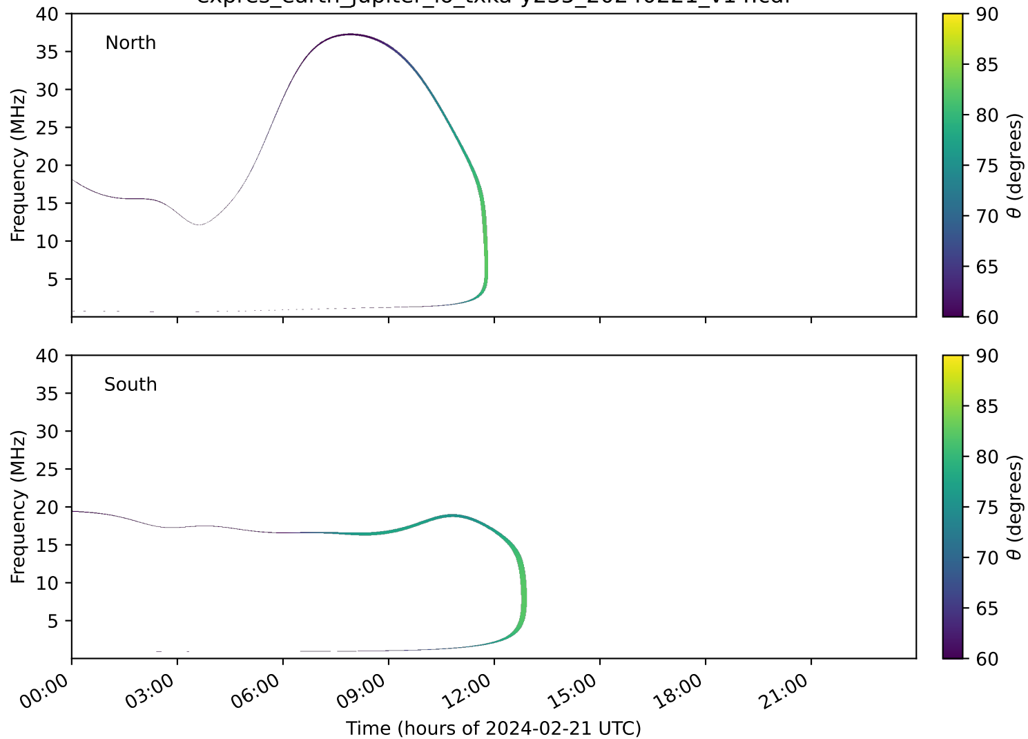
expres_earth_jupiter_io_txka-y235_20240221_v14.cdf
