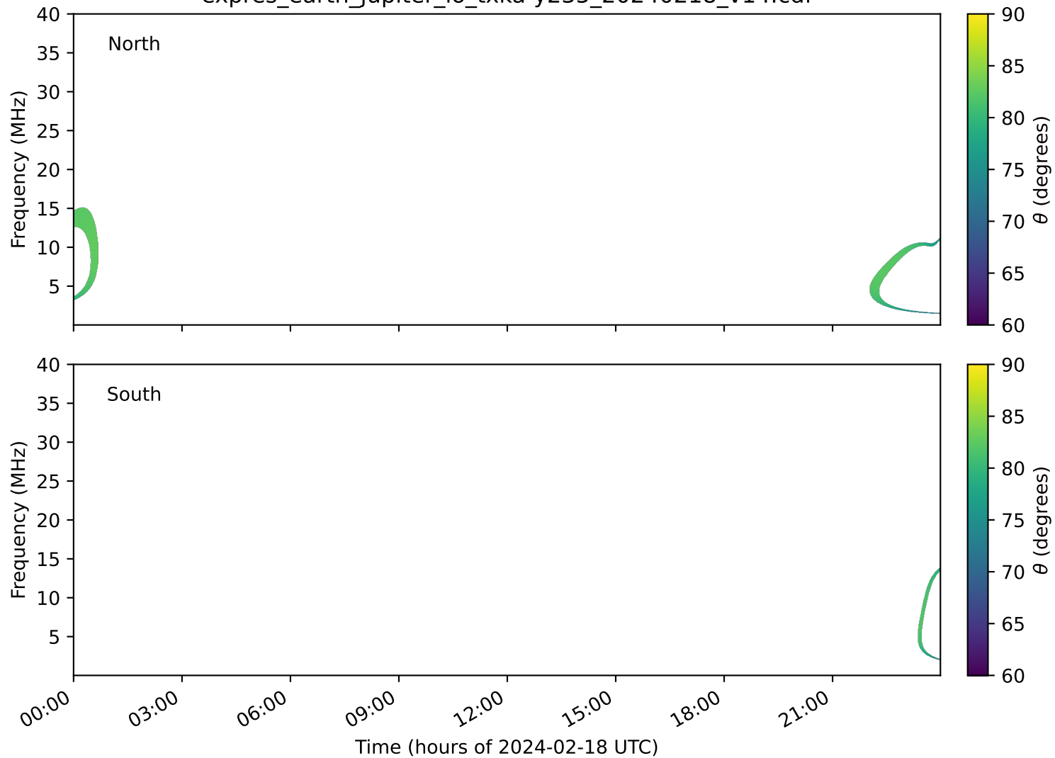
expres_earth_jupiter_io_txka-y235_20240218_v14.cdf
