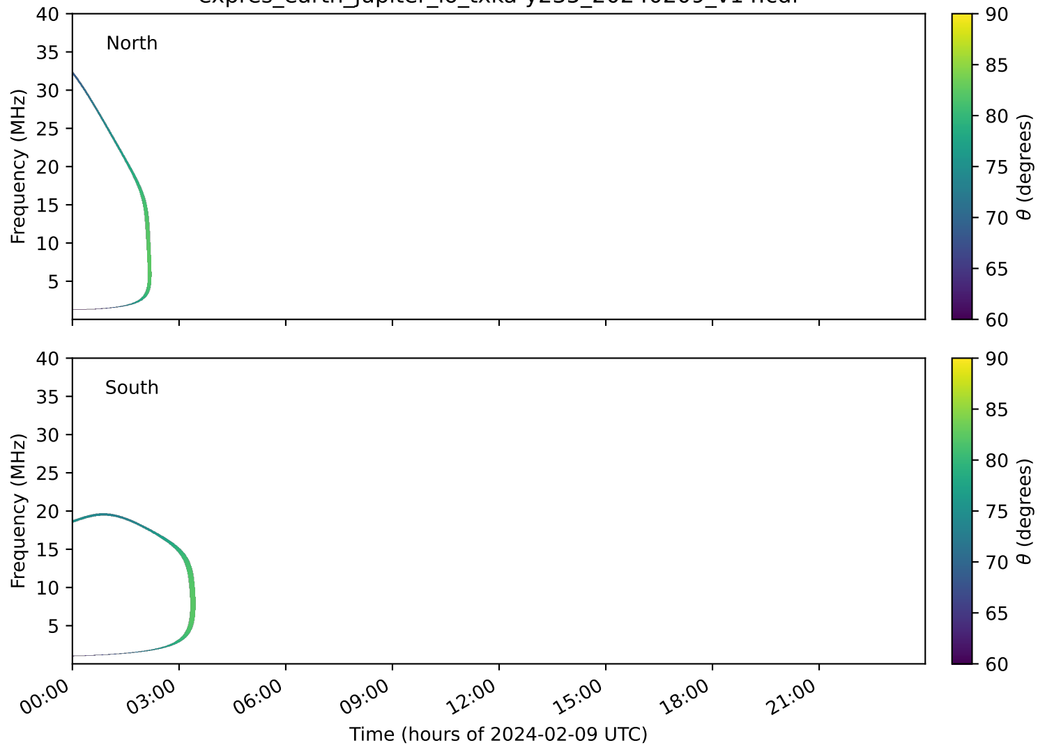
expres_earth_jupiter_io_txka-y235_20240209_v14.cdf
