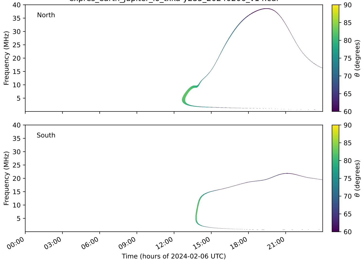
expres_earth_jupiter_io_txka-y235_20240206_v14.cdf
