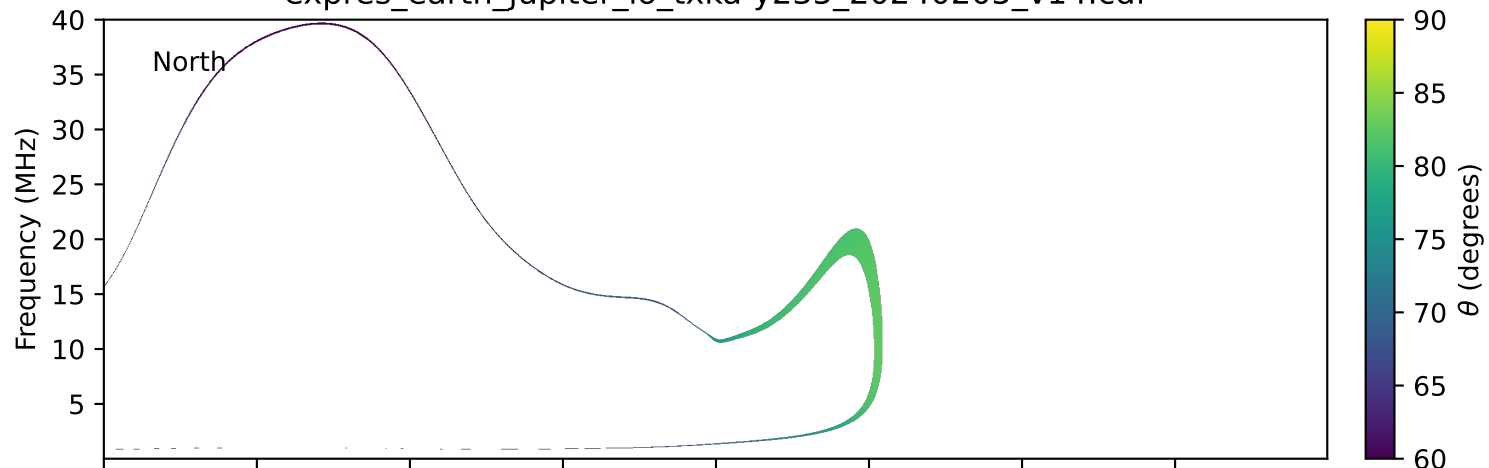
expres_earth_jupiter_io_txka-y235_20240205_v14.cdf
