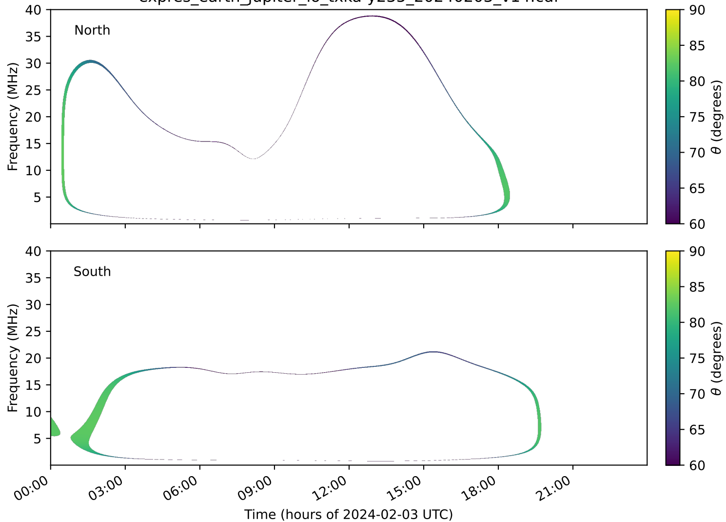
expres_earth_jupiter_io_txka-y235_20240203_v14.cdf
