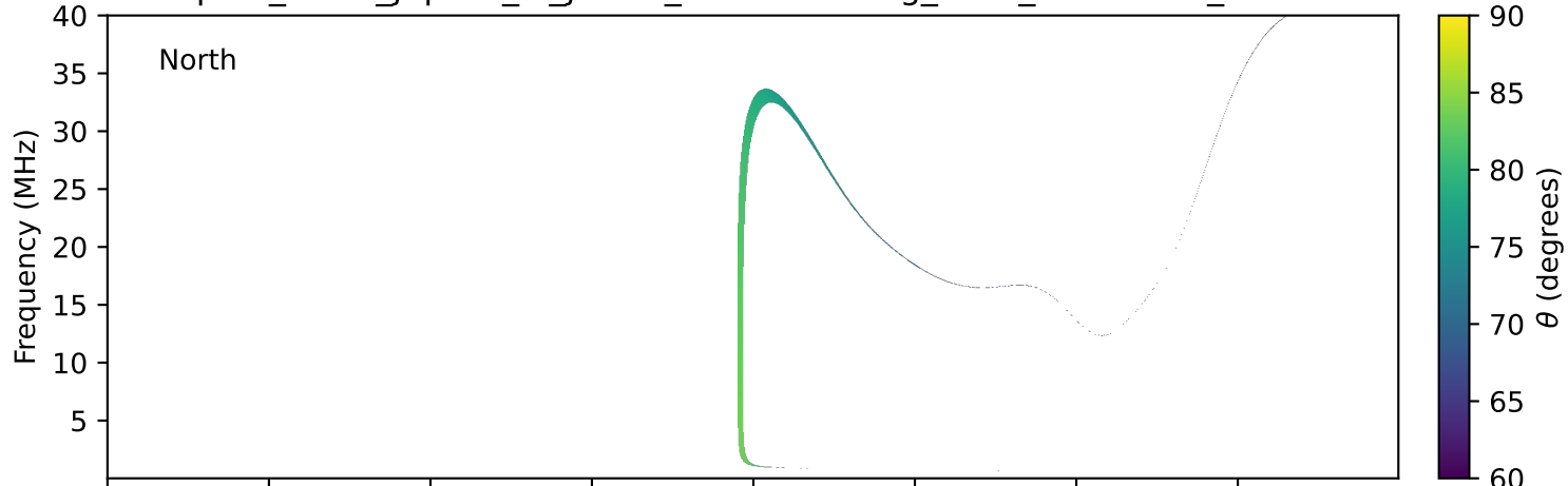
expres_earth_jupiter_io_jrm33_lossc-wid1deg_3kev_20240222_v11.cdf
