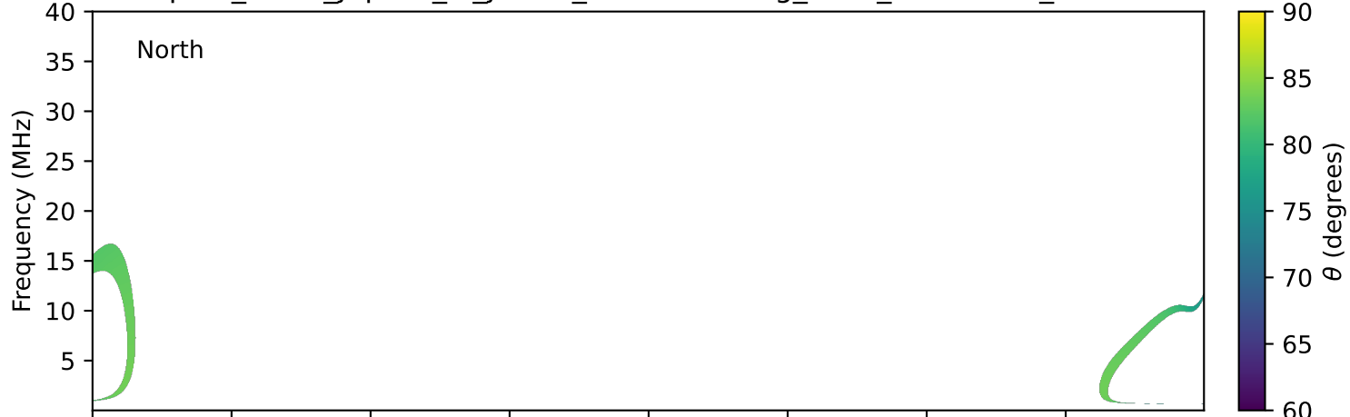
expres_earth_jupiter_io_jrm33_lossc-wid1deg_3kev_20240218_v11.cdf
