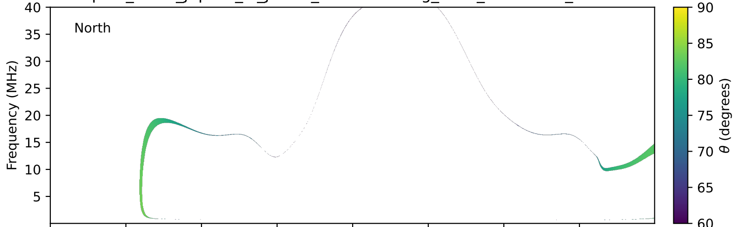
expres_earth_jupiter_io_jrm33_lossc-wid1deg_3kev_20240217_v11.cdf
