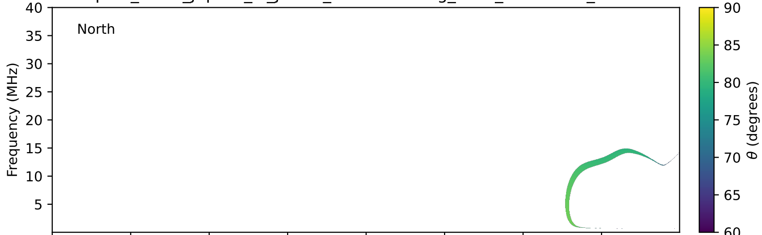
expres_earth_jupiter_io_jrm33_lossc-wid1deg_3kev_20240211_v11.cdf
