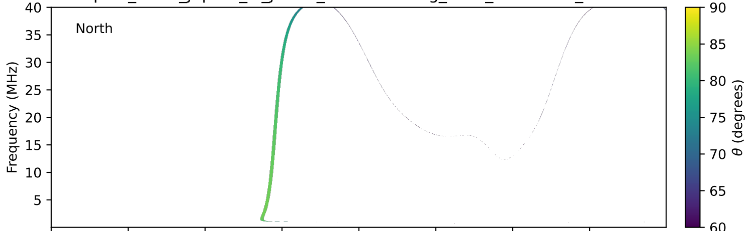
expres_earth_jupiter_io_jrm33_lossc-wid1deg_3kev_20240208_v11.cdf
