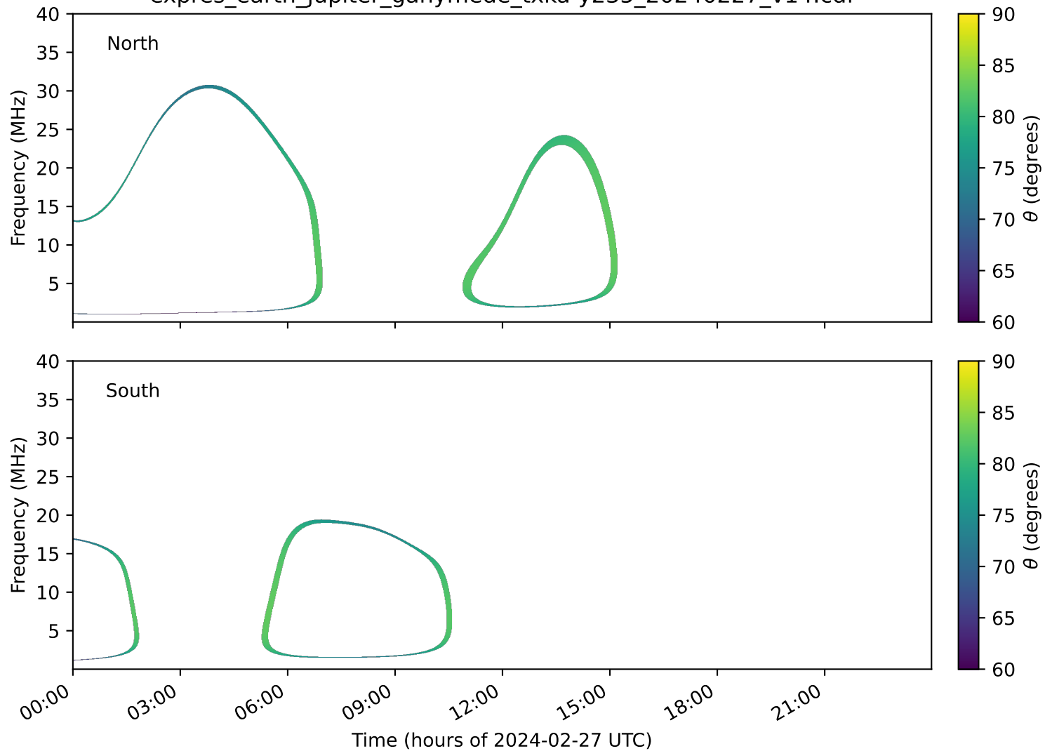
expres_earth_jupiter_ganymede_txka-y235_20240227_v14.cdf
