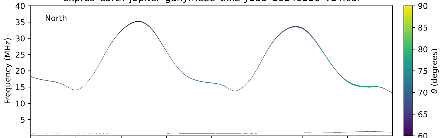
expres_earth_jupiter_ganymede_txka-y235_20240226_v14.cdf
