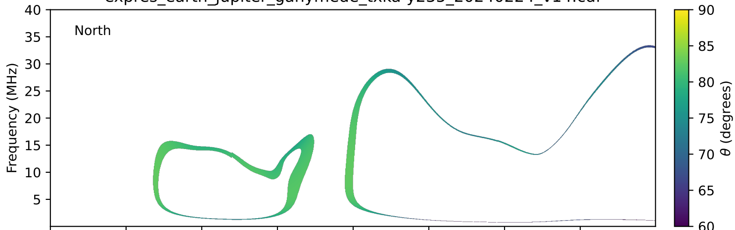
expres_earth_jupiter_ganymede_txka-y235_20240224_v14.cdf
