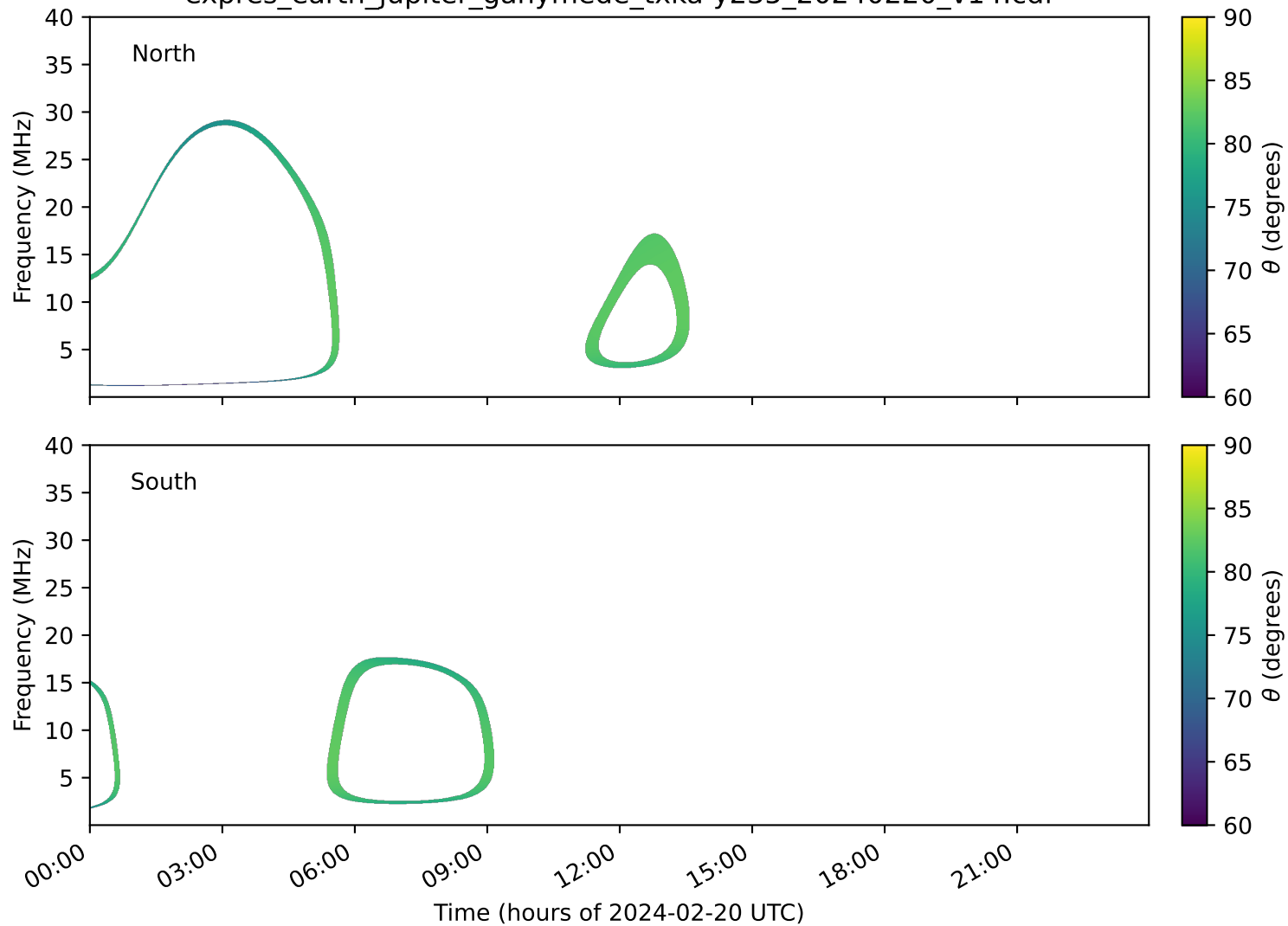
expres_earth_jupiter_ganymede_txka-y235_20240220_v14.cdf
