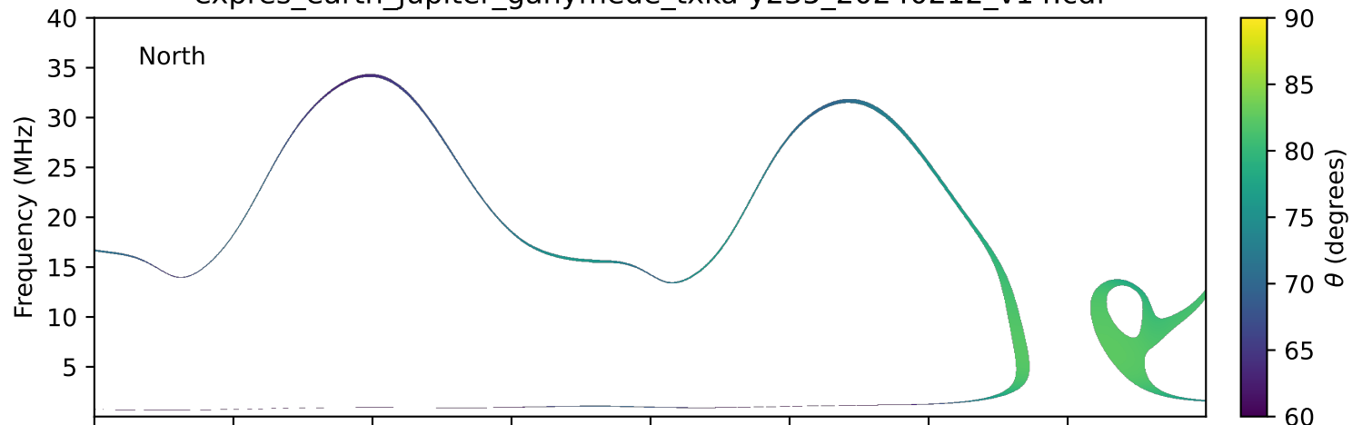
expres_earth_jupiter_ganymede_txka-y235_20240212_v14.cdf
