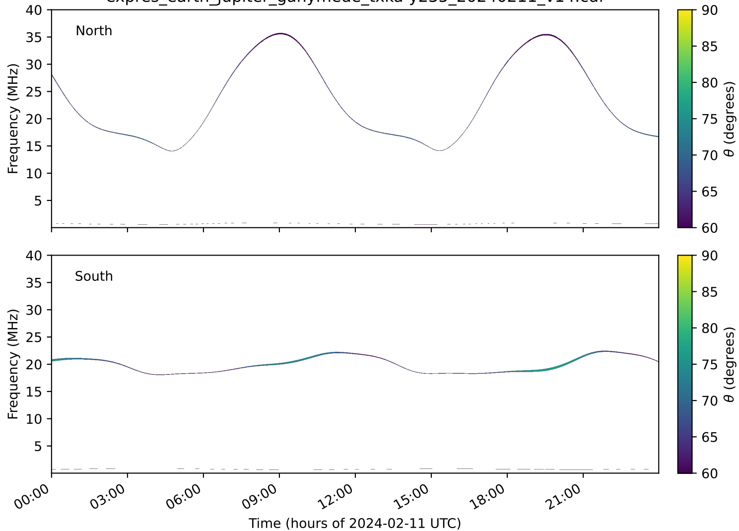
expres_earth_jupiter_ganymede_txka-y235_20240211_v14.cdf
