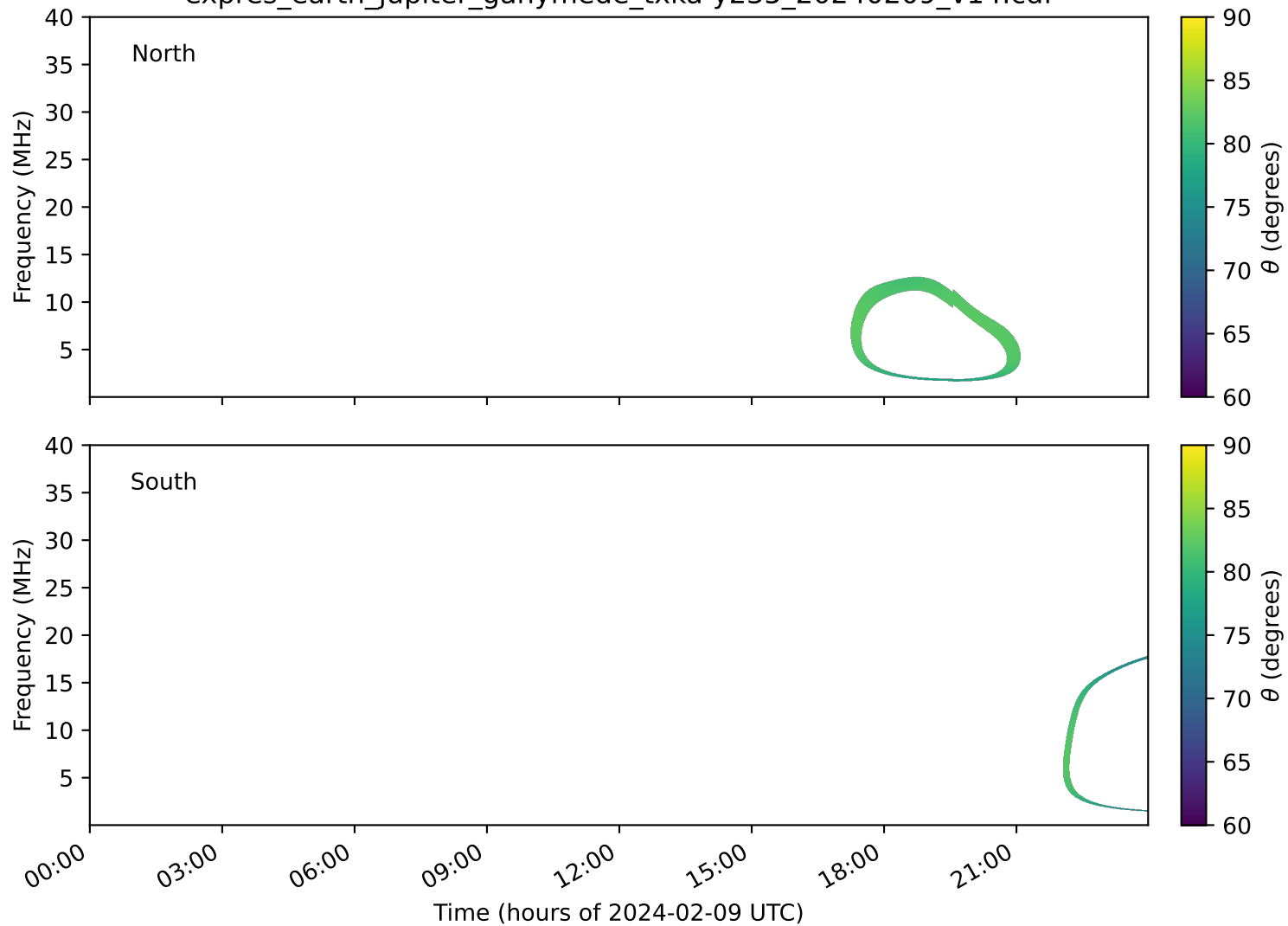
expres_earth_jupiter_ganymede_txka-y235_20240209_v14.cdf
