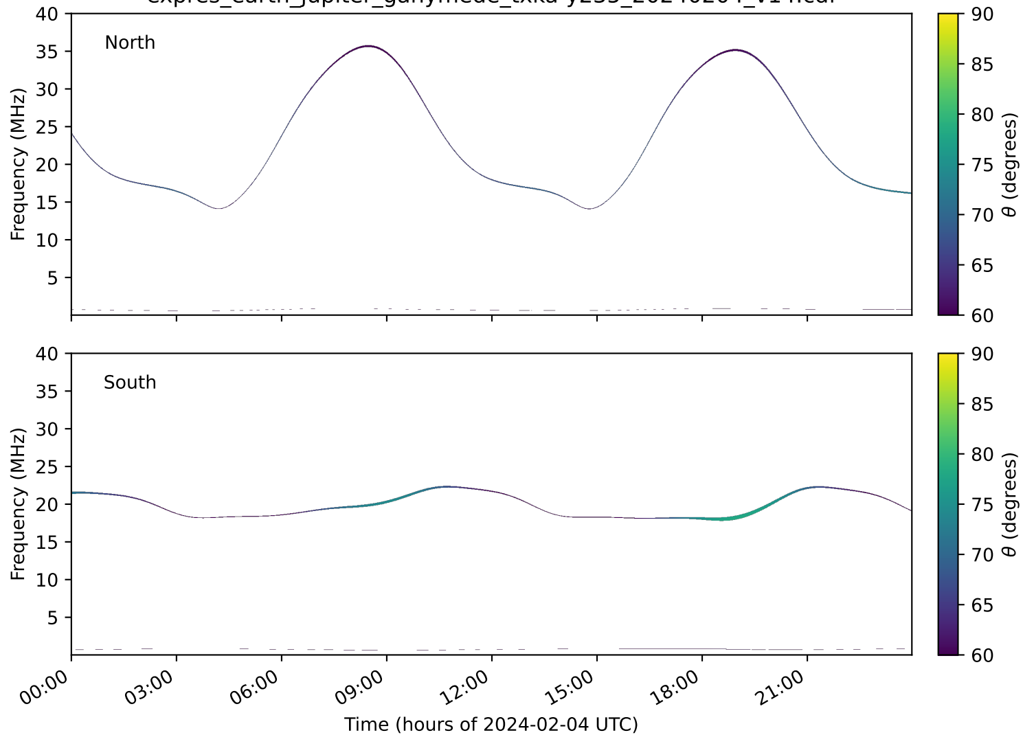
expres_earth_jupiter_ganymede_txka-y235_20240204_v14.cdf
