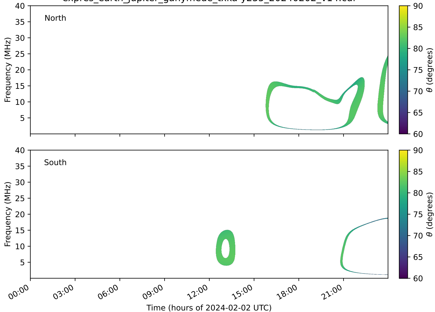
expres_earth_jupiter_ganymede_txka-y235_20240202_v14.cdf
