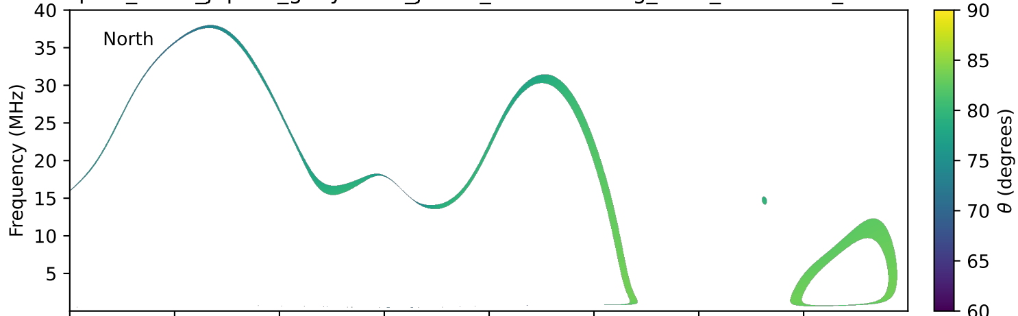
expres_earth_jupiter_ganymede_jrm33_lossc-wid1deg_3kev_20240227_v11.cdf
