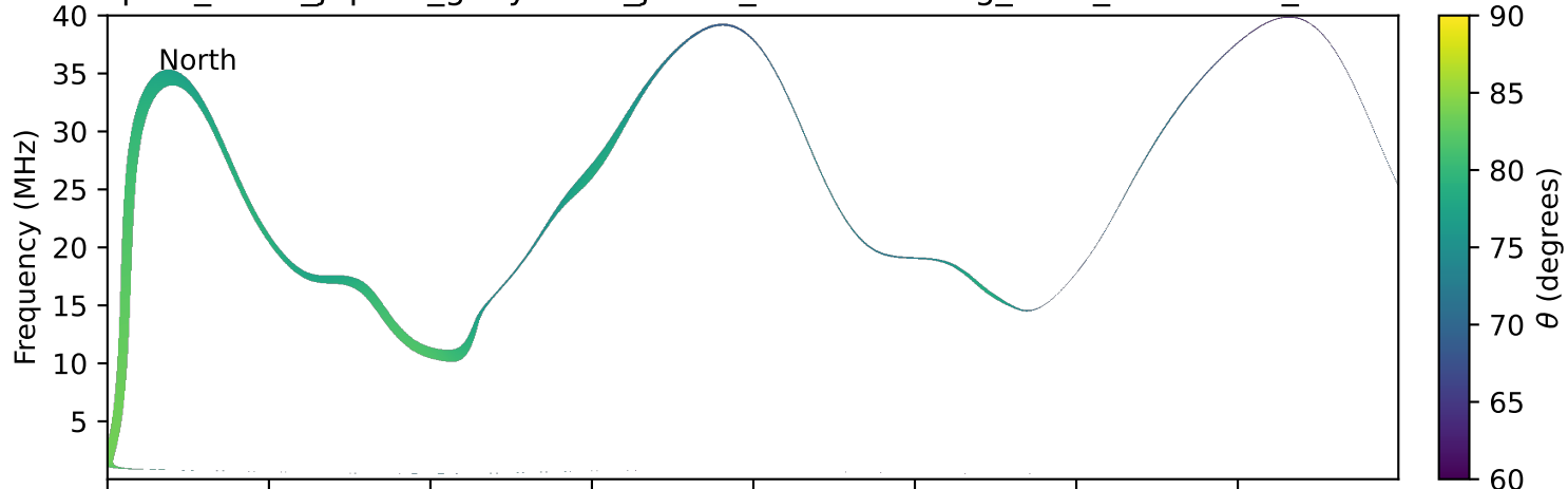
expres_earth_jupiter_ganymede_jrm33_lossc-wid1deg_3kev_20240203_v11.cdf
