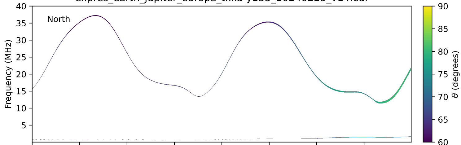
expres_earth_jupiter_europa_txka-y235_20240229_v14.cdf
