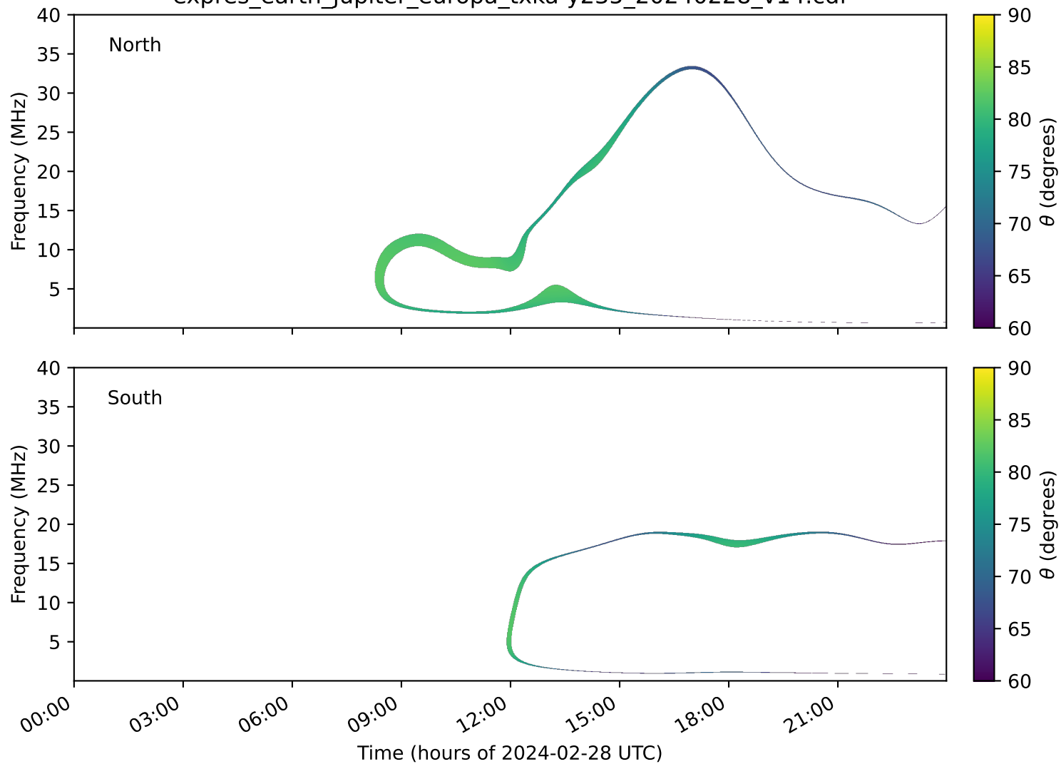
expres_earth_jupiter_europa_txka-y235_20240228_v14.cdf
