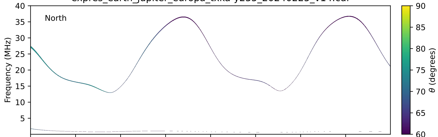
expres_earth_jupiter_europa_txka-y235_20240225_v14.cdf
