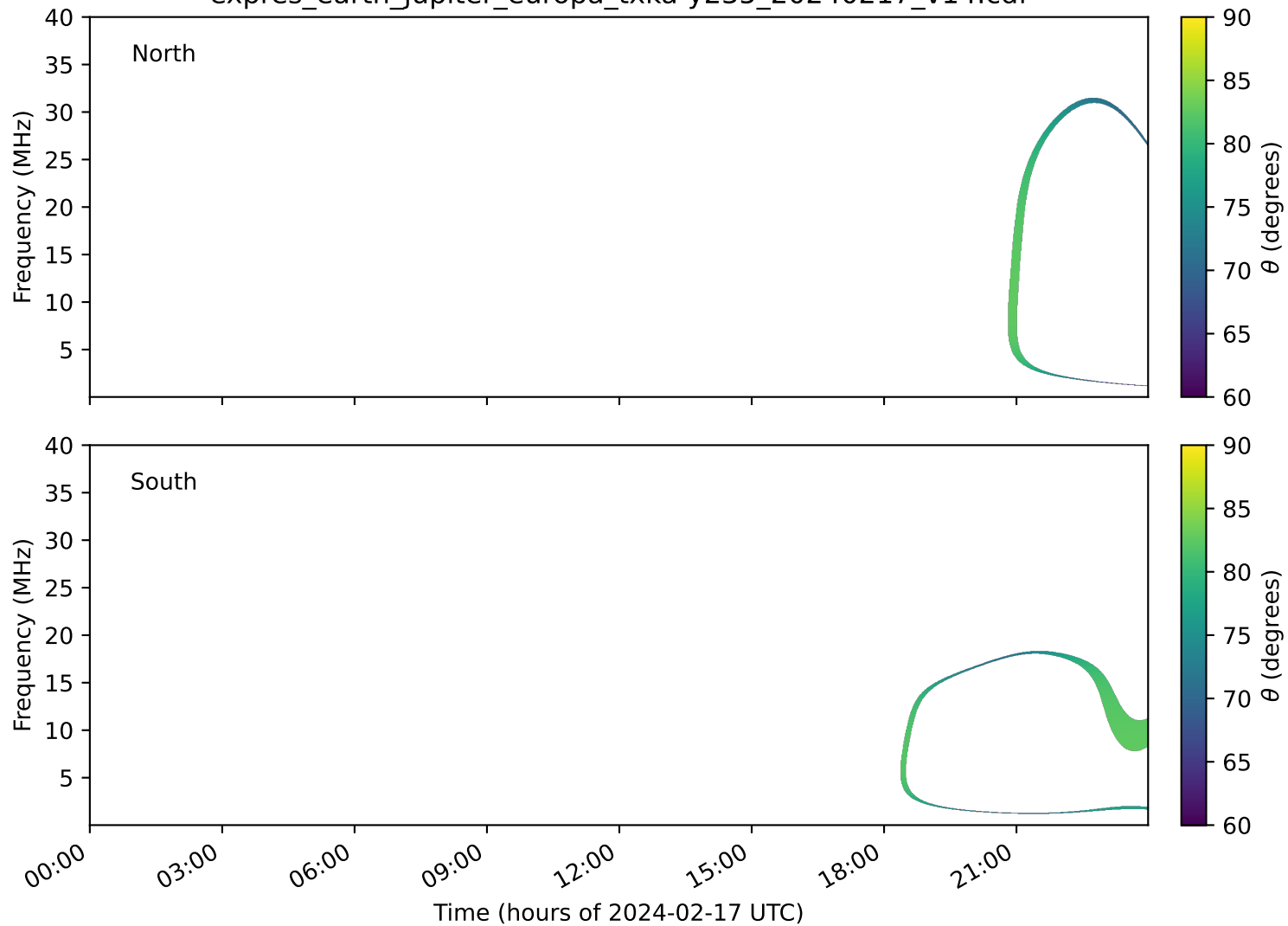
expres_earth_jupiter_europa_txka-y235_20240217_v14.cdf
