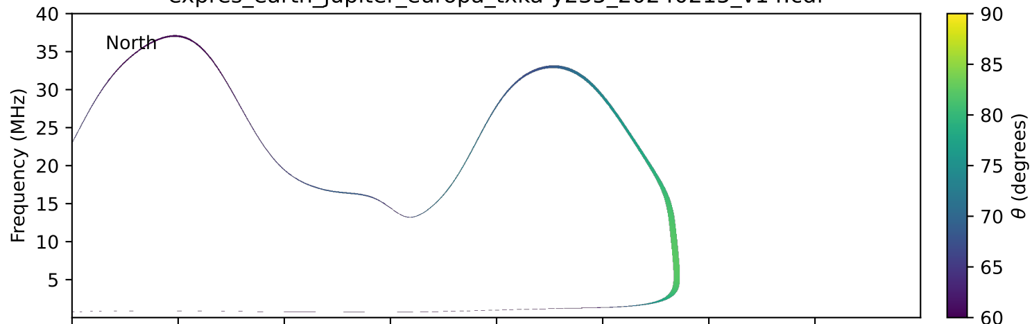
expres_earth_jupiter_europa_txka-y235_20240215_v14.cdf
