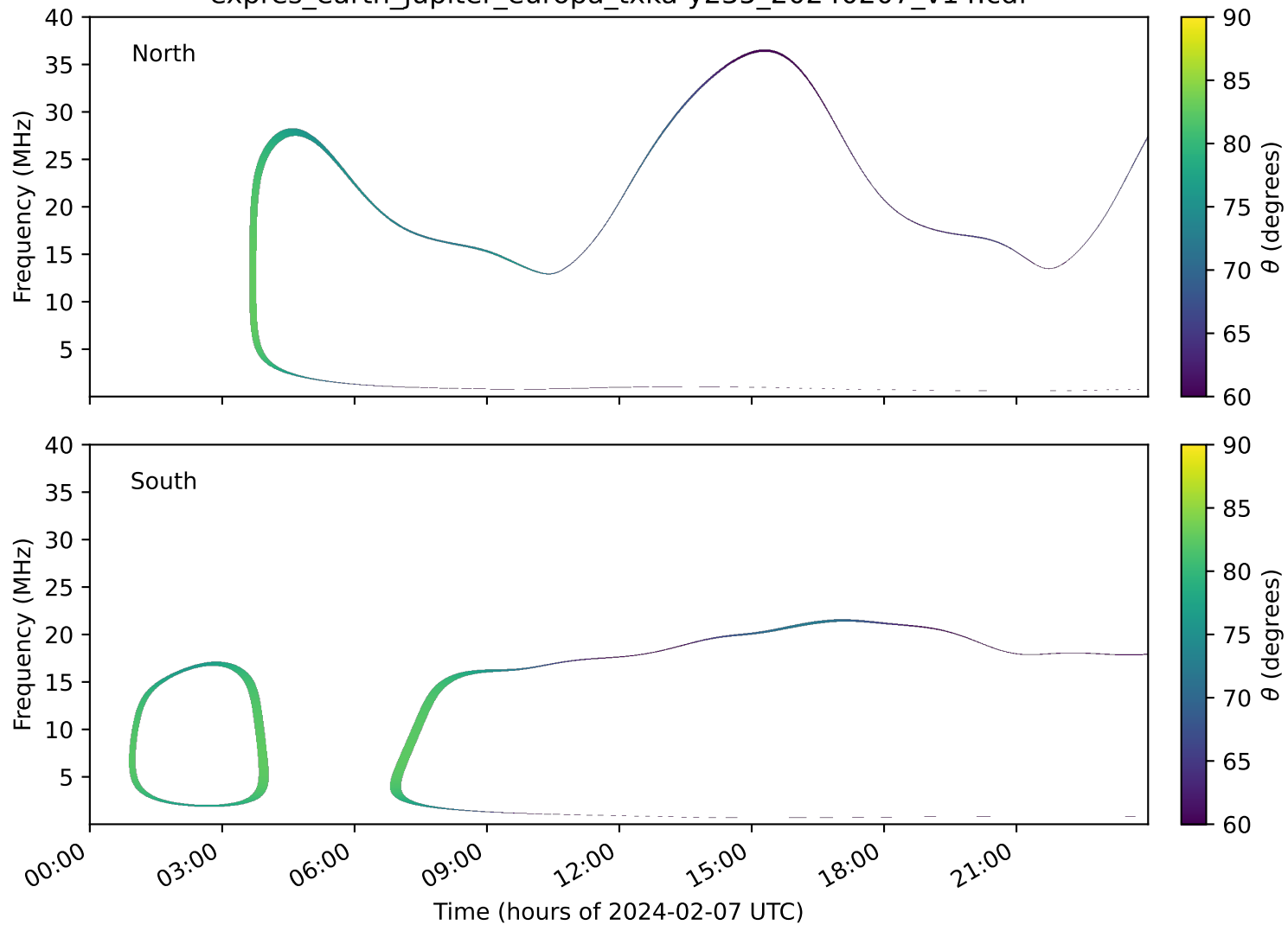
expres_earth_jupiter_europa_txka-y235_20240207_v14.cdf
