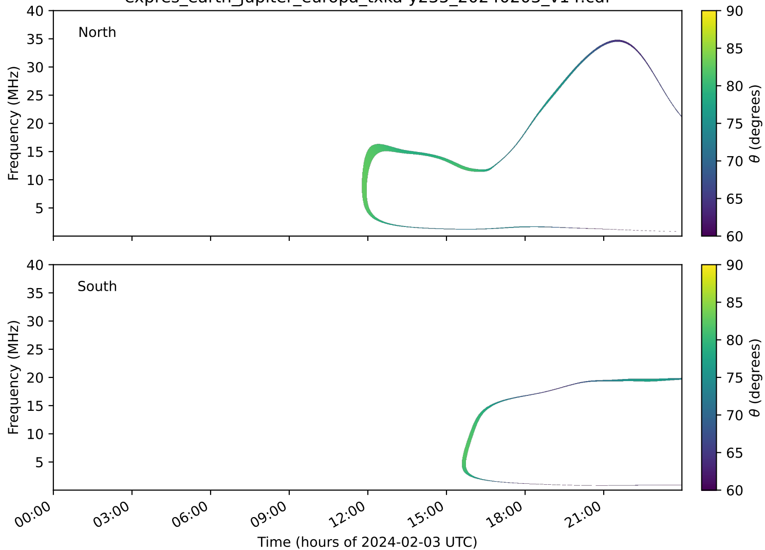
expres_earth_jupiter_europa_txka-y235_20240203_v14.cdf
