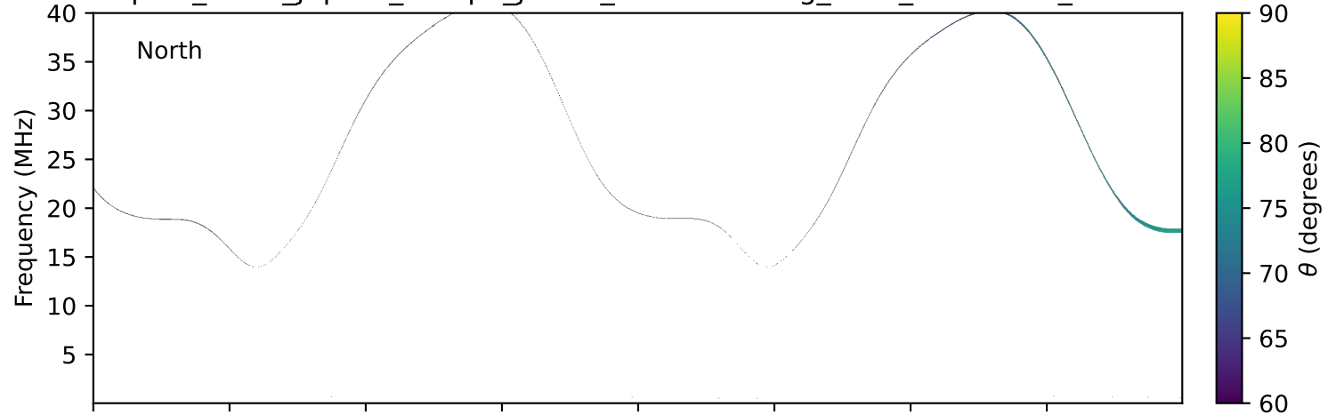
expres_earth_jupiter_europa_jrm33_lossc-wid1deg_3kev_20240204_v11.cdf
