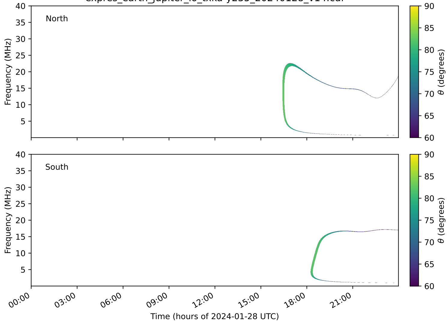
expres_earth_jupiter_io_txka-y235_20240128_v14.cdf
